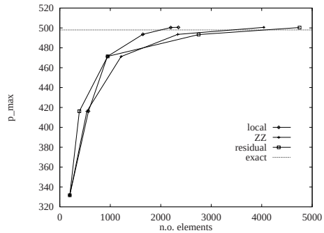
Fig. 8.8 Convergence behaviour
