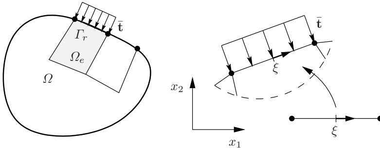
Fig. 4.10 (a) Surface load
