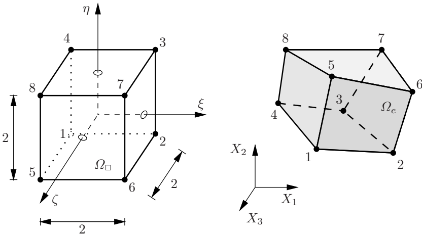
Fig. 4.8 Isoparametric 8-node hexahedral element
