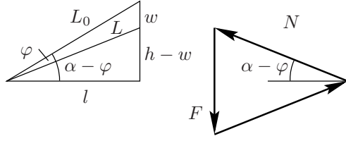
Fig. 2.7b Geometry and equilibrium
