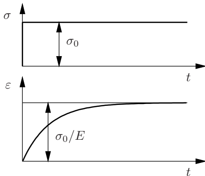
Fig. 3.9b Creep process
