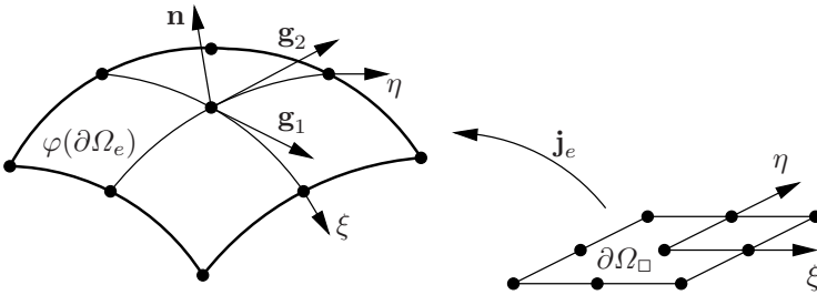
Fig. 4.13 Coordinate systems for deformation dependent loads
