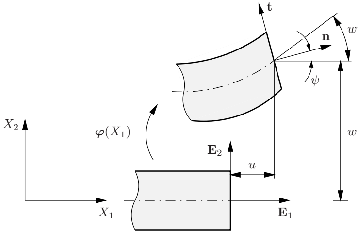
Fig. 9.6 Beam kinematics
