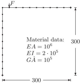
Fig. 9.9 Frame structure
