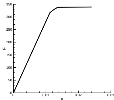
Fig. 9.3b Load–displacement curve of the truss structure
