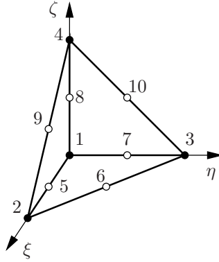
Fig. 4.9 Isoparametric 4 and 10 node tetrahedral
