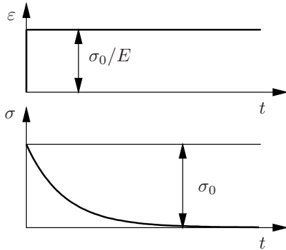
Fig. 3.10b Relaxation
