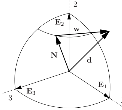
Fig. 9.18 Parametrization of the extensible director \mathbf{d}
