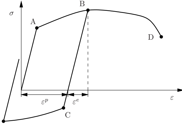
Fig. 3.6 Elasto-plastic constitutive behaviour
