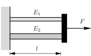
Fig. 2.9a System and loading
