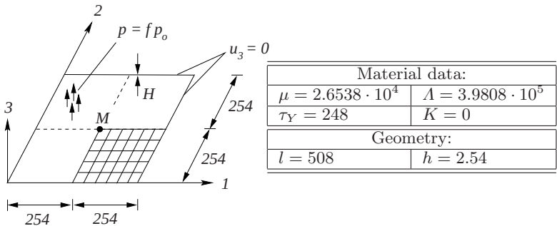
Fig. 9.23 Quadratic plate under internal pressure
