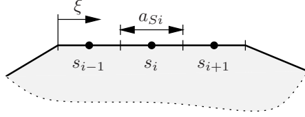
Fig. 11.7 Multiple slave nodes on one segment
