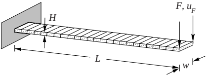
Fig. 9.21 Bending of a clamped beam
