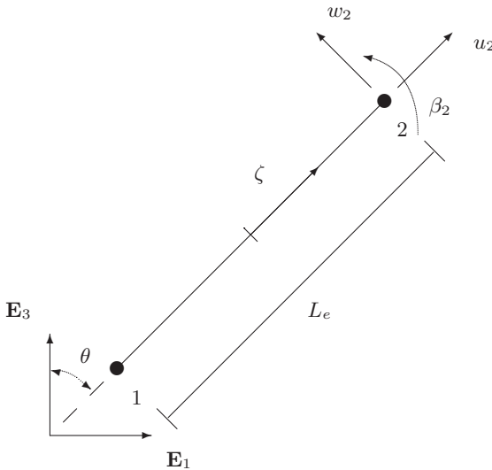
Fig. 9.13 3-parameter-shell element
