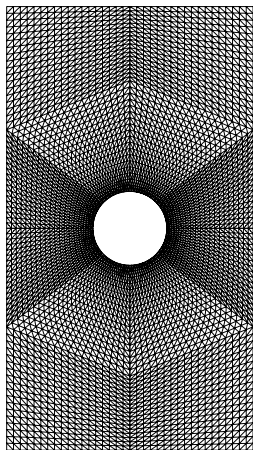
Fig. 5.25 Plate with hole with elasto-plastic material
