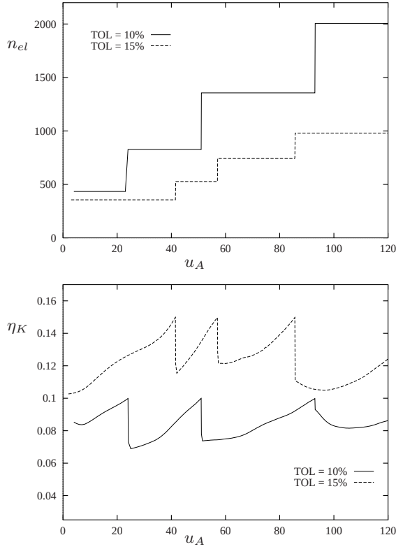
Fig. 8.14 Strategy I: Number of used elements and relative error of the adaptive computation
