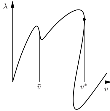
Fig. 5.8 Displacement control
