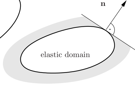
Fig. 3.7b Admissible region
