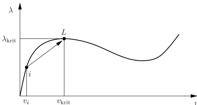
Fig. 7.3 Direct method for the computation of a singular point
