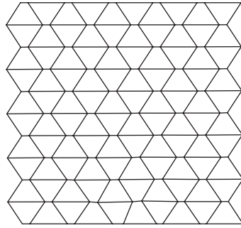
Fig. 10.2b Hourglass eigenvector
