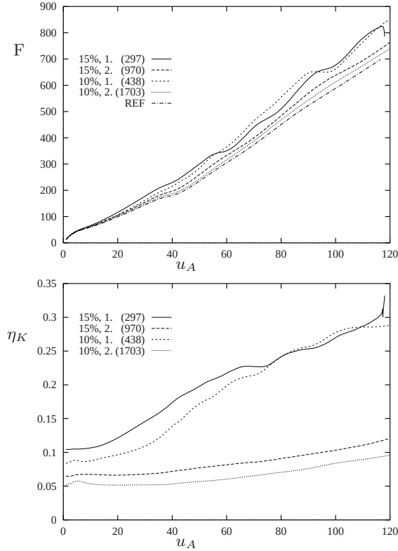
Fig. 8.16 Strategy II: Load–displacement curve, energy norm \|\boldsymbol{\tau}\|_K and relative error
