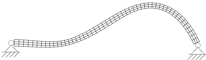
Fig. 7.6 Eigenform of the arc at bifurcation point B
