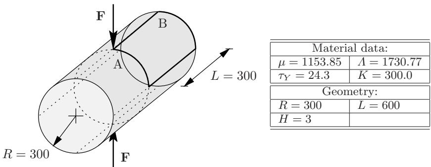
Fig. 9.25 Pinched cylinder
