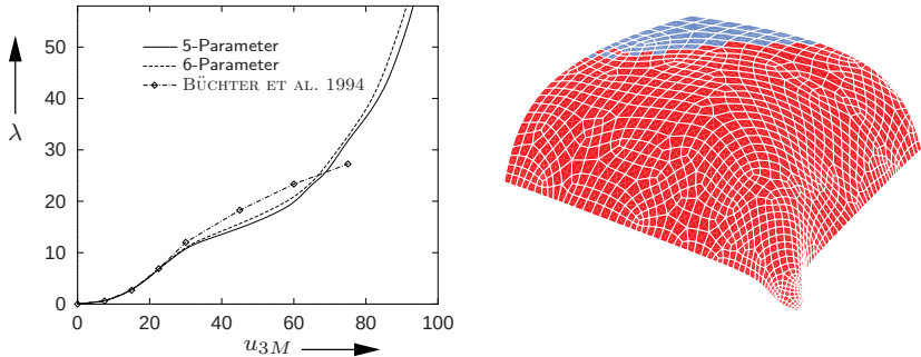
Fig. 9.24 Load-deflection curves and deformed configuration at \lambda = 70
