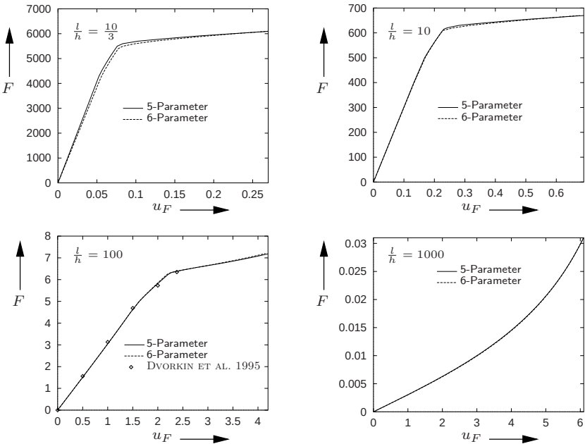
Fig. 9.22 Load–deflection curves
