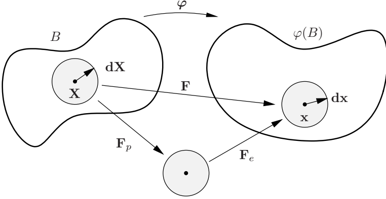
Fig. 3.8 Multiplicative decomposition of the deformation gradient \mathbf{F}
