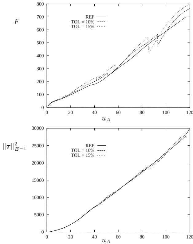
Fig. 8.13 Strategy I: Load–deflection curve and energy norm \|\tau\|_{E-1}^2 .
