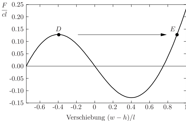
Fig. 2.8 Load–deflection curve
