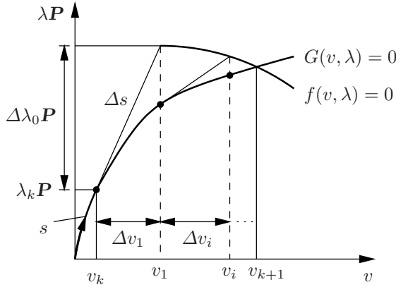
Fig. 5.6 Arc-length method
