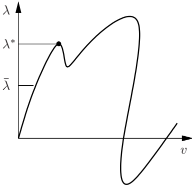
Fig. 5.7 Load control
