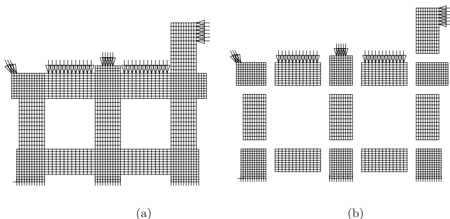
Fig. 5.28 (a) Structure and loading, (b) Distribution of the mesh onto 14 processors using subdomains
