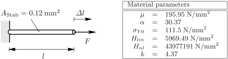
Fig. 9.4 One-dimensional elasto-plastic truss model for polymer strings
