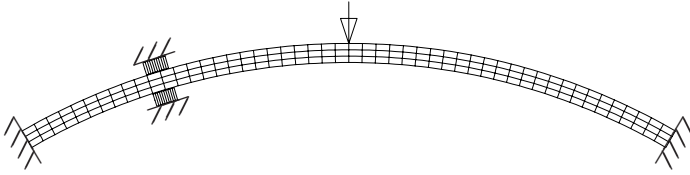
Fig. 5.15 FE-discretization of the arc
